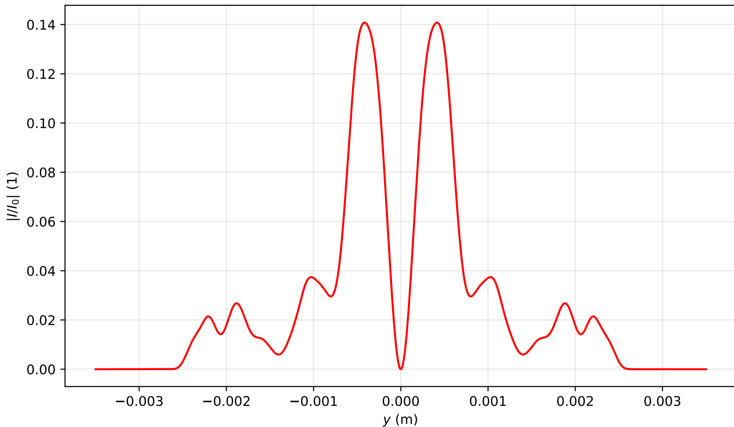
Intensity profile I(x = 0, y, z = 3.742)/I_0 , P_{in}=8.0P_{cr} , artificial time
